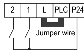
Source logic
