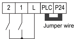
Sink logic
